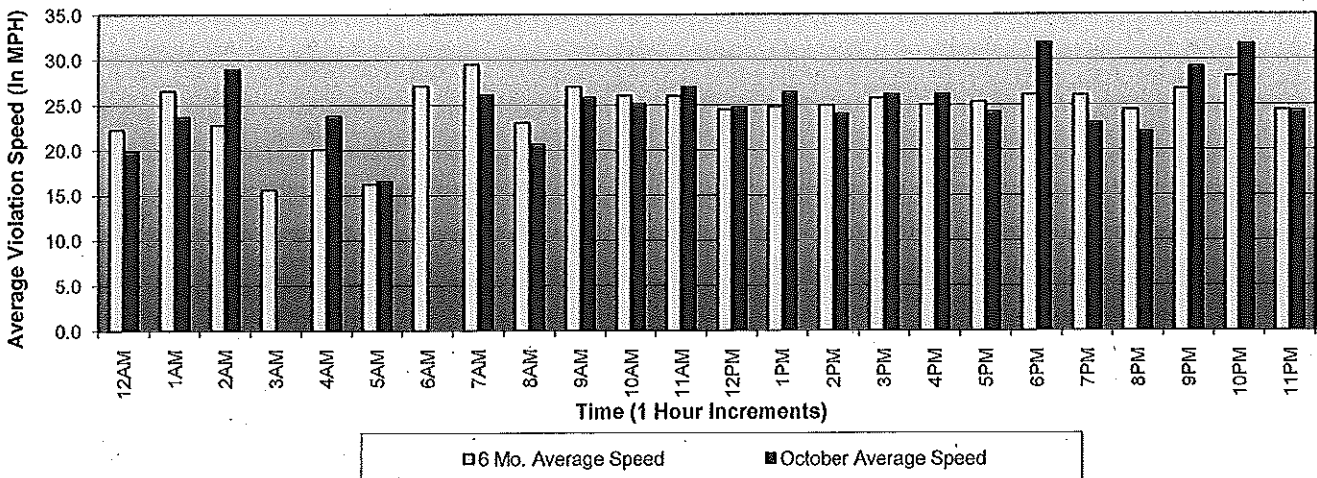
Average Violation Speed (Weekends, 6 Mo. Trend, May - October)
